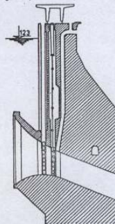
S1.14.6. Detalj ulaza na HE Salakovac
